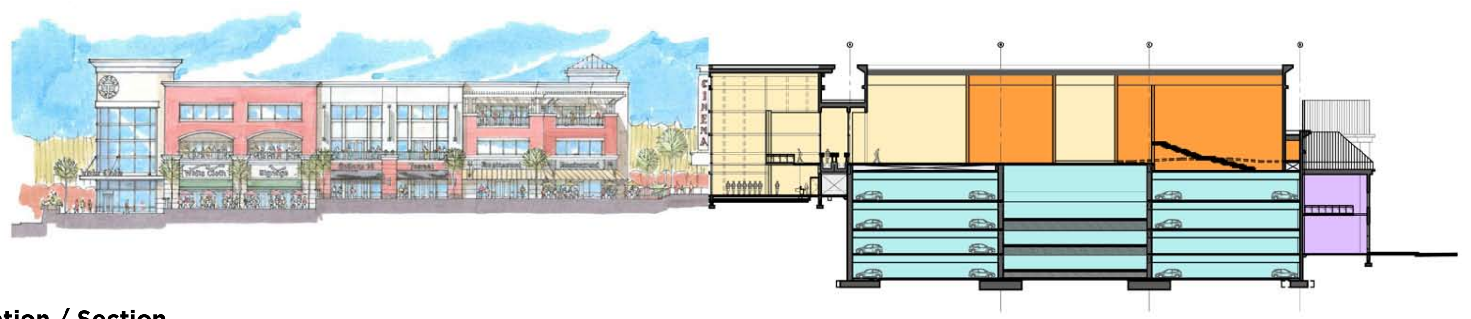
East Elevation / Section View from Plaza
